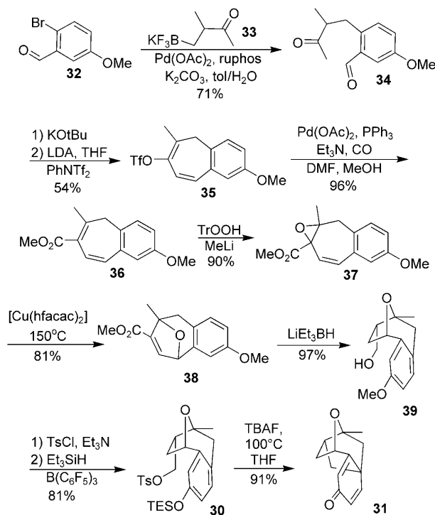
Scheme 5. Efficient synthesis of the platensimycin core. ruphos = 2-dicyclohexylphosphino-2',6'-diisopropoxybiphenyl.
